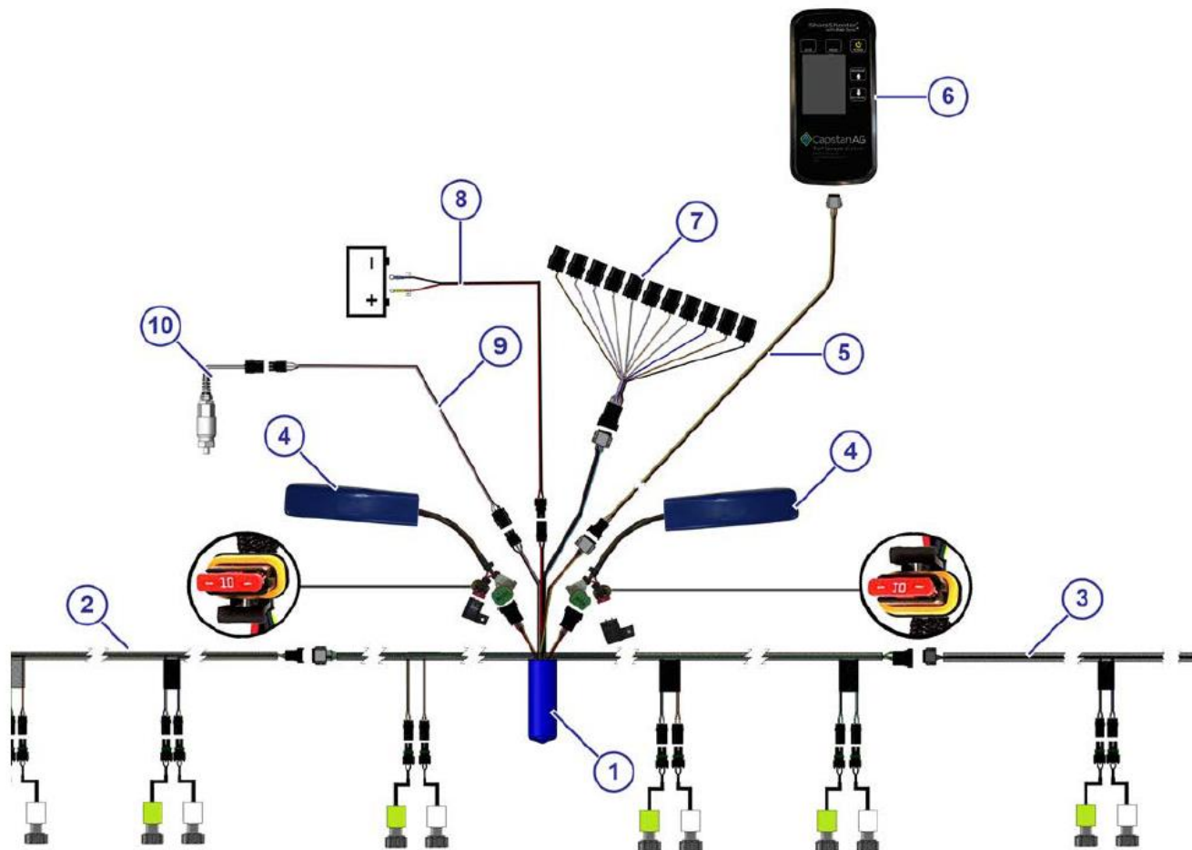
Capstan General Layout
